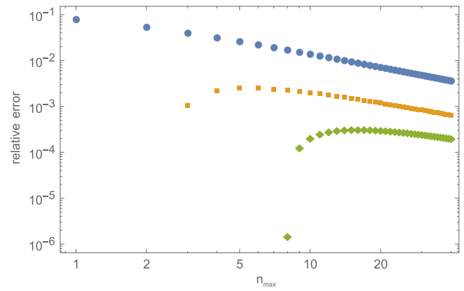
Figure 3. Relative error in logarithmic scale for very large number of electronic shells for TF approximation and the approximations including second- and fourth-order terms of gradient expansion. The markers are the same as in figure 2. Since the asymptotic dependence is linear with the tangent (-1) in all cases, it shows that the relative errors at large Z are proportional to Z^{-1/3} in all cases.
